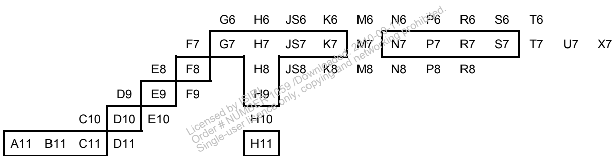
Figure 10 — Holes
